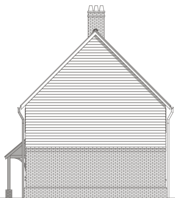
SIDE ELEVATION
